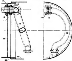
Figs. 368-369. Dry Pipe and Steam Pipe Connections
